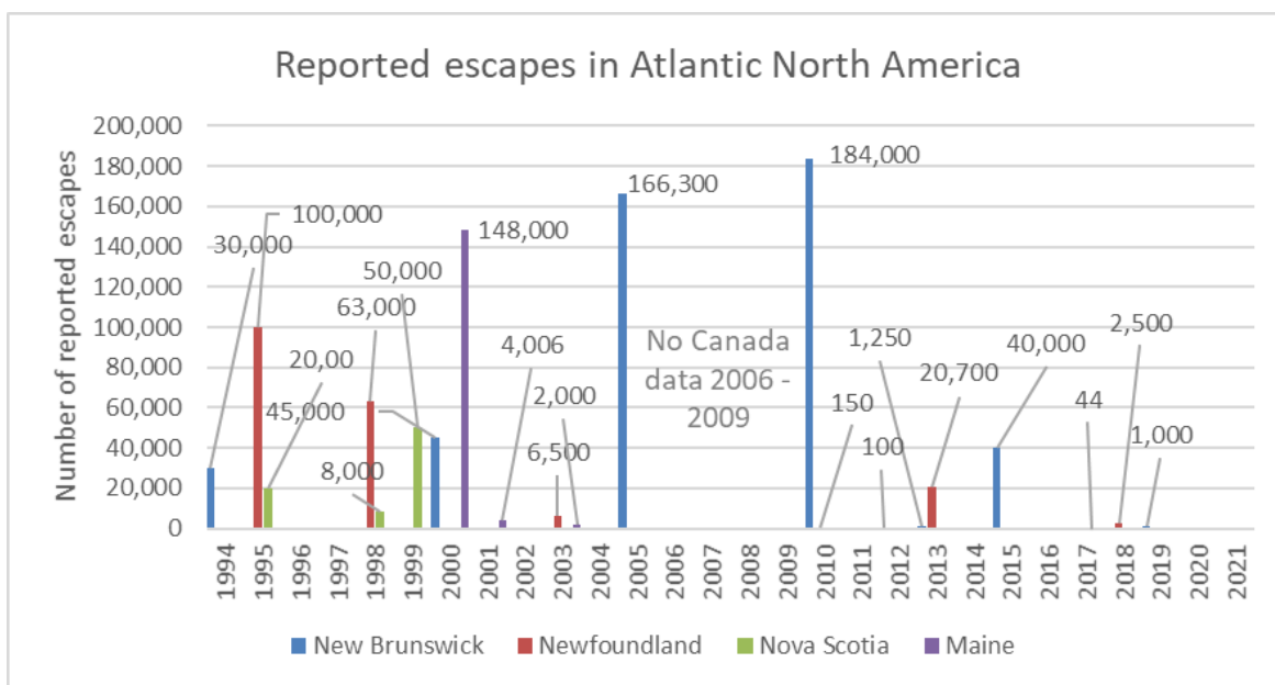
Figure 24: Escape data compiled from DFO, Maine DMR and media searches (see text above for references). Note where a range of escape numbers was listed, the median value was used here.
