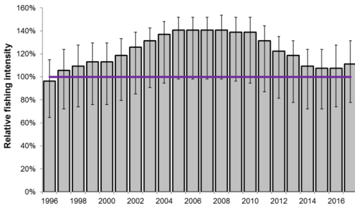
Figure 68 Recent estimated fishing intensity (based on the Spawning Potential Ratio) relative to the SPR=46% reference level (horizontal line). Vertical lines indicate approximate credible intervals from the stock assessment ensemble (Steward & Hicks 2017).
