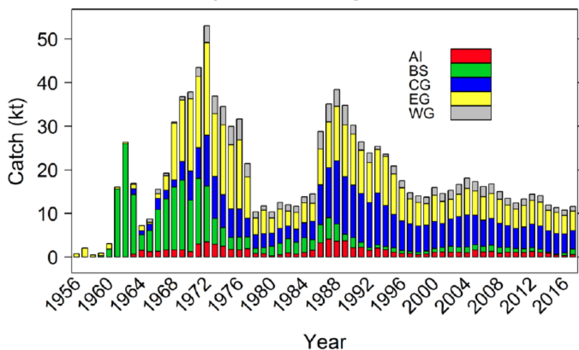
Figure 54 Sablefish fishery total reported catch (kt) by North Pacific Fishery Management Council area and year (Hanselman et al. 2017).
