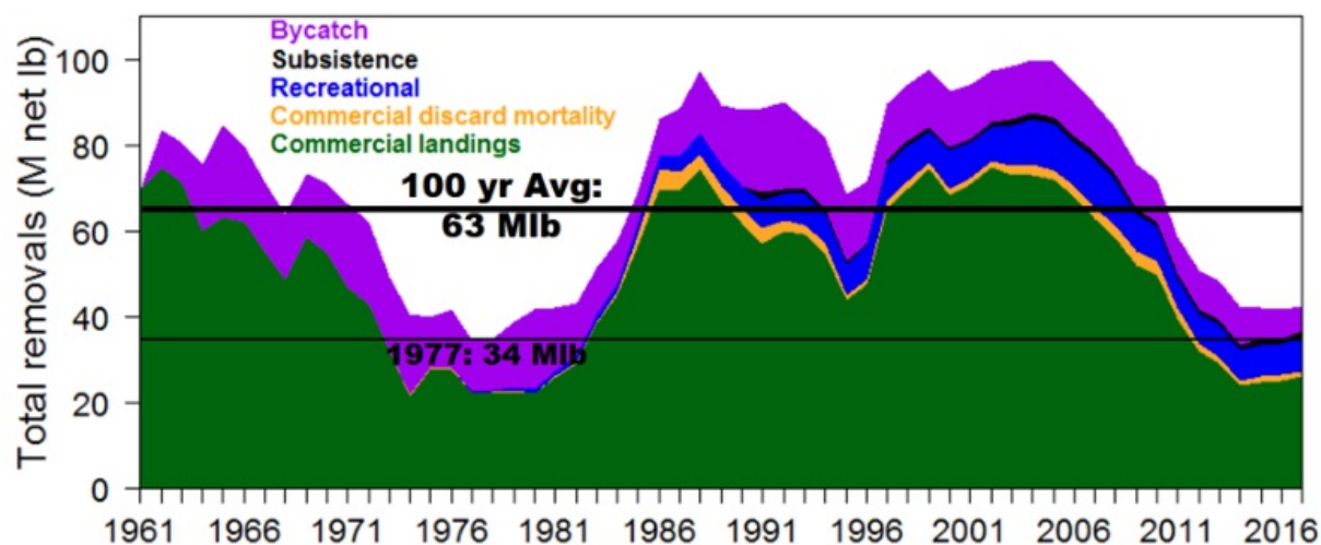
Figure 72 Total removals coastwide for the period 1961-2016 (IPHC 2017).
