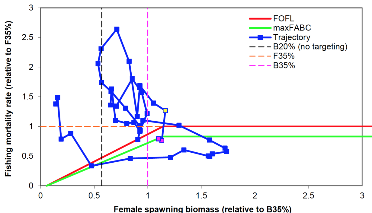
Figure 39 Trajectory of Pacific cod fishing mortality and spawning biomass based on the most current 2017 model, 1977-2019 (yellow square = 2018, magenta squares = 2019 and 2020)(Thompson 2017)..
