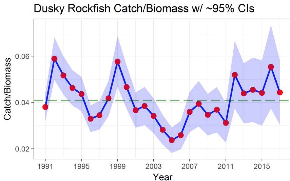
Figure 18 GOA Dusky rockfish catch/biomass ratio with approximate 95% confidence intervals. Green dashed line is long-term average for the time series. Biomass is age 4+ biomass from the age structured assessment model (Fenske et al. 2017).
