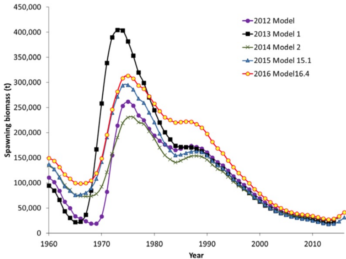
Figure 13 Female spawning biomass in tons for BSAI Greenland Turbot for Model 16.4 and previous years' stock assessments (Barbeaux et al. 2016).
