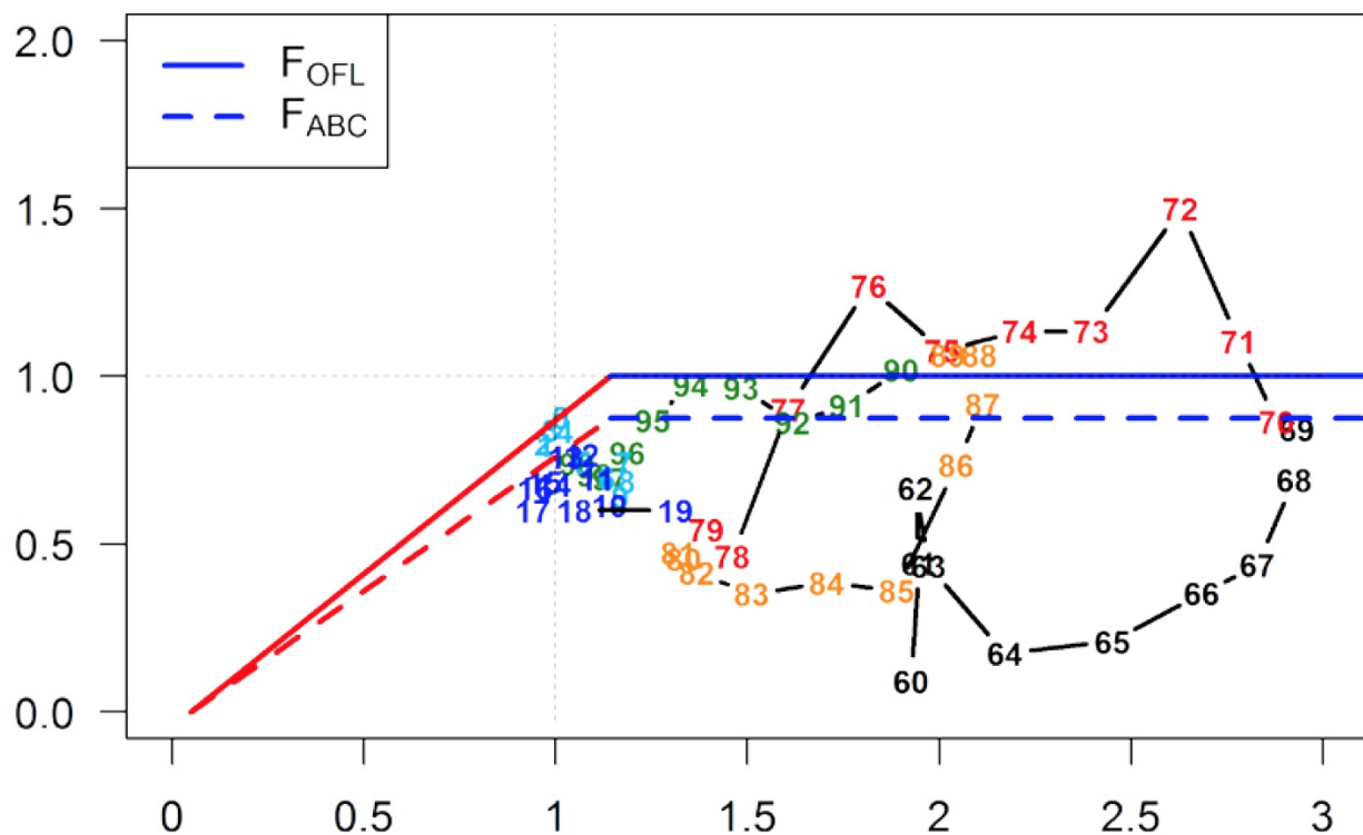
Figure 59 Phase-plane diagram of time series of sablefish estimated spawning biomass relative to the unfished level and fishing mortality relative to FOFL for author recommended model. Y-axis represents F/F_{35\%} . X-axis represents SSB/B_{35\%} (Hanselman et al. 2017).
