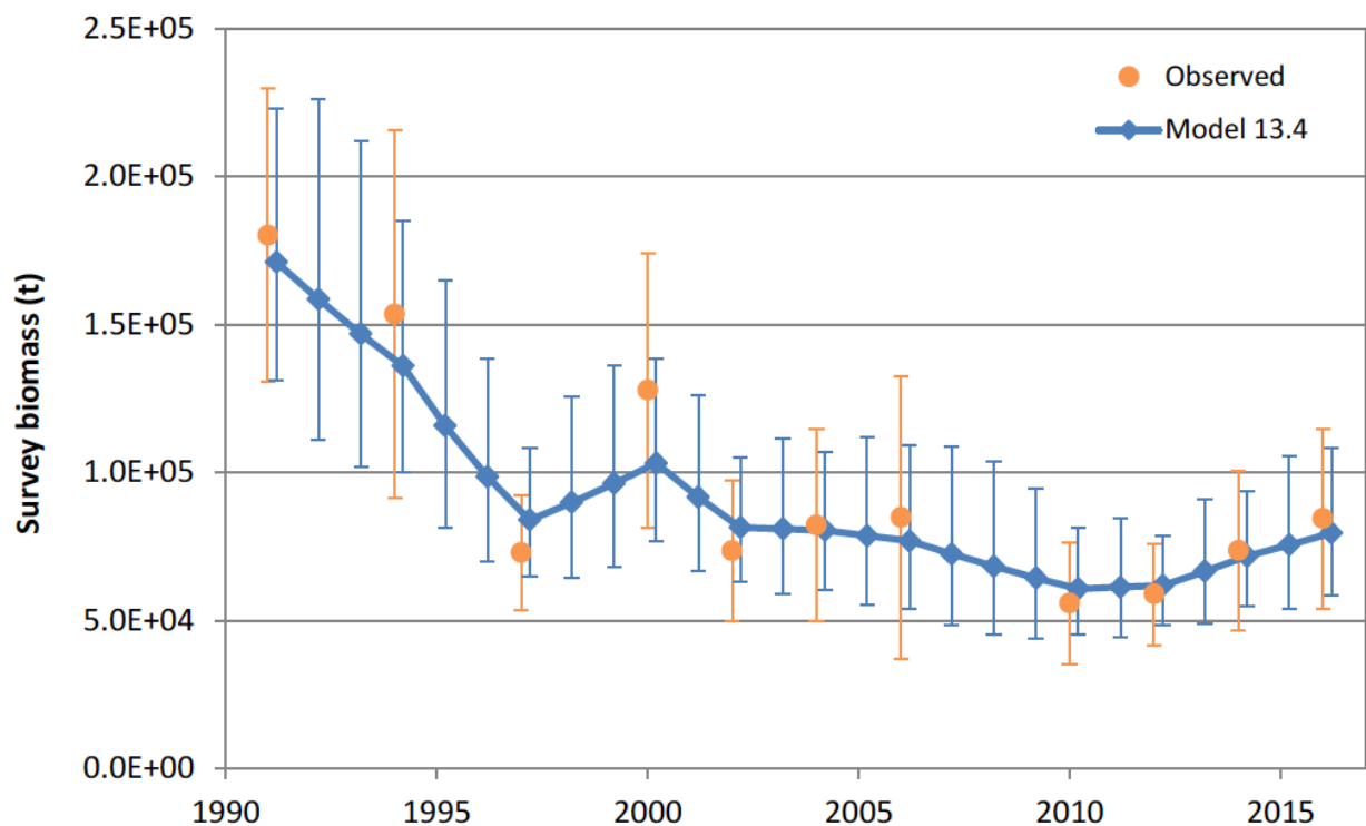
Figure 43 Fit of model to survey AI Pacific cod biomass time series, with 95% confidence intervals for the observations and estimates (Thomson & Pálsson 2017).
