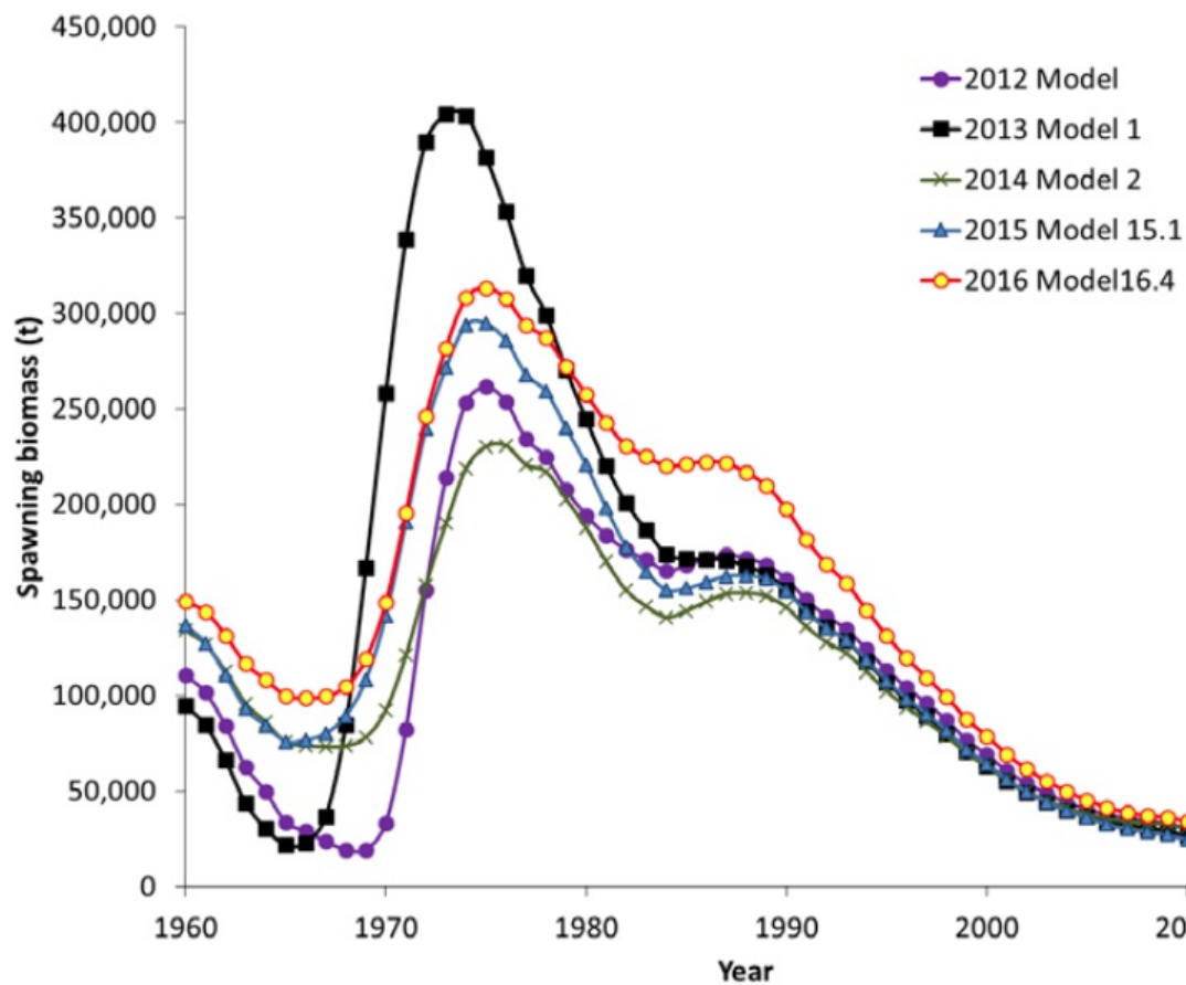
Figure 10 Female spawning biomass in tons for BSAI Greenland Turbot for Model 16.4 and previous years' stock assessments (Barbeaux et al. 2016).
