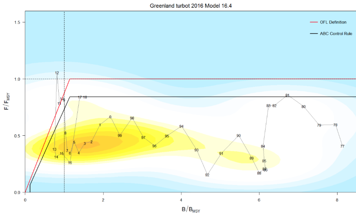
Figure 12 For Model 16.4 ratio of historical F/F_{MSY} versus female spawning biomass relative to B_{MSY} for BSAI Greenland turbot, 1977-2018. Note that the proxies for F_{MSY} and B_{MSY} are F_{35\%} and B_{35\%} , respectively. The F_s presented are the sum of the full F_s across fleets (Barbeaux et al. 2016).
