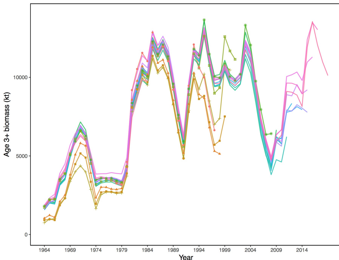
Figure 63 Comparison of the current assessment results with past assessments of begin-year EBS age-3+ pollock biomass (Ianelli et al. 2017).
