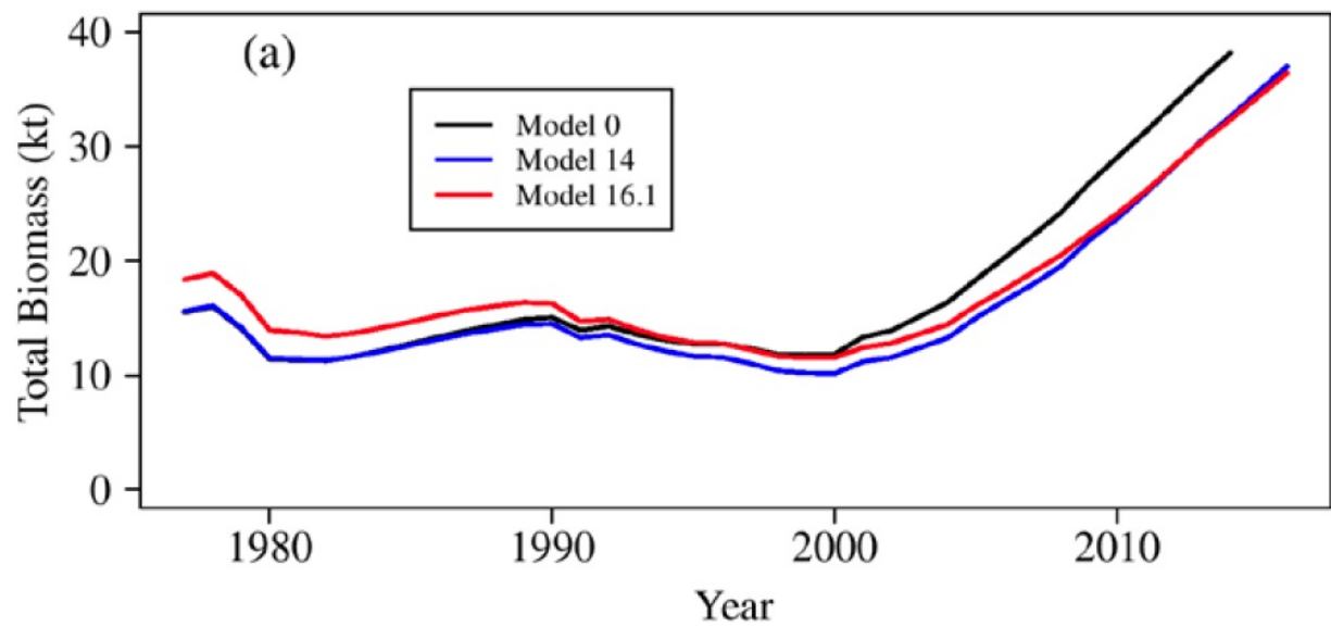
Figure 8 Estimated BSAI blackspotted and rougheye rockfish complex total biomass (Spencer & Rooper 2016).
