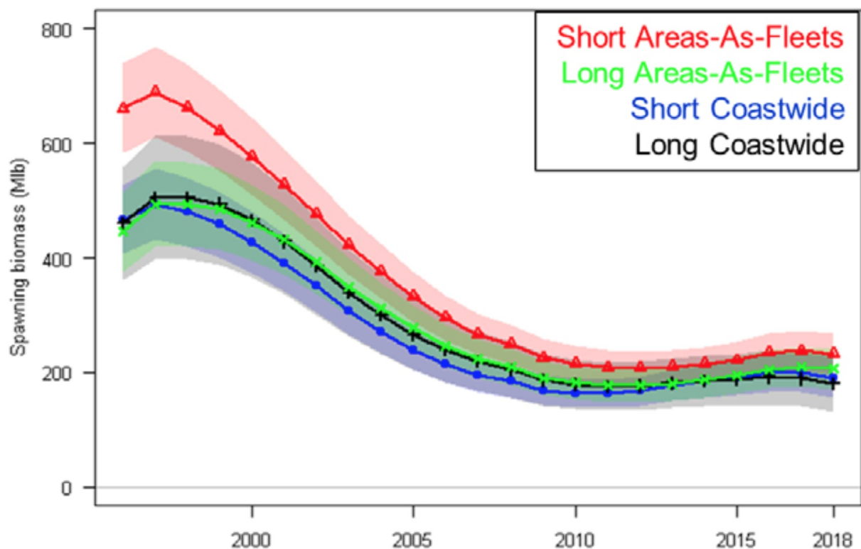
Figure 66 Estimated spawning biomass trends (1996-2018) based on the four individual models included in the
