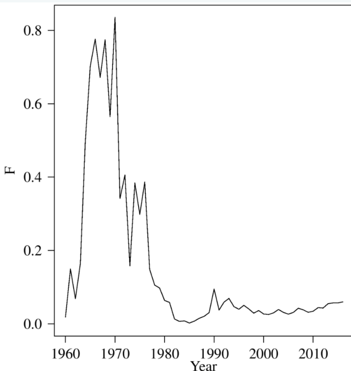
Figure 49 Estimated fully selected fishing mortality for BSAI POP (Spencer & Ianelli 2016).
