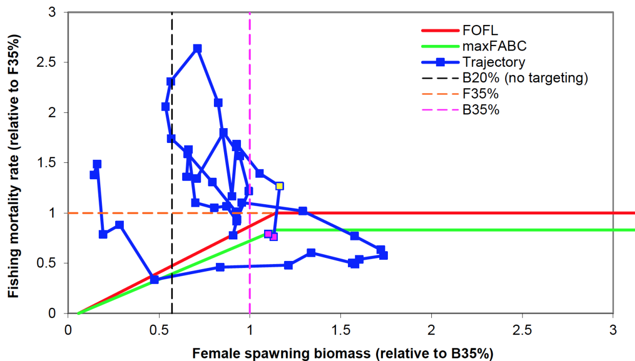
Figure 31 Trajectory of Pacific cod fishing mortality and spawning biomass based on the most current 2017 model, 1977-2019 (yellow square = 2018, magenta squares = 2019 and 2020)(Thompson 2017)..
