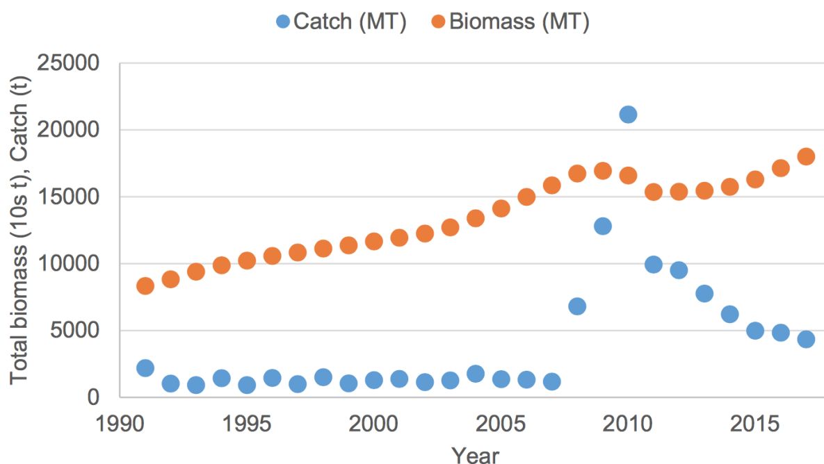
Figure 64 Time series of total biomass (10s of tons), catch (tons) of kamchatka flounder (Bryan & Wilderbuer 2017).
