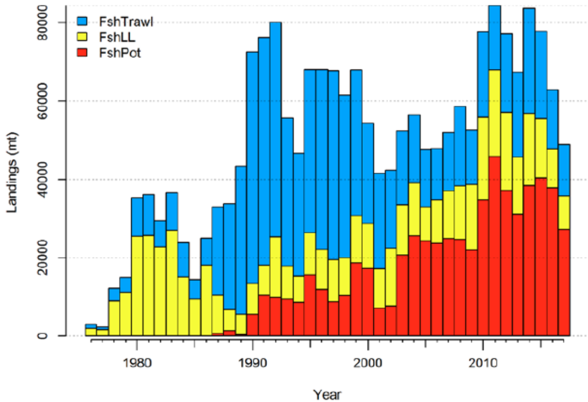
Figure 28 GOA Pacific cod catch from 1977-2017 (2017 estimated)(Barbeaux et al. 2017).
