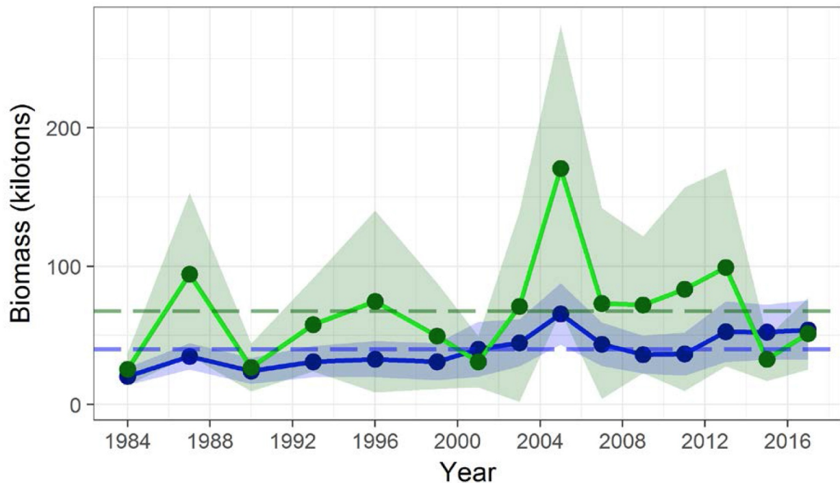
Figure 17 Comparison of dusky rockfish abundance estimates from Gulf of Alaska trawl survey using the geostatistical abundance estimator (blue) and the design based estimator (green), with approximate 95% confidence intervals (Fenske et al. 2017).
