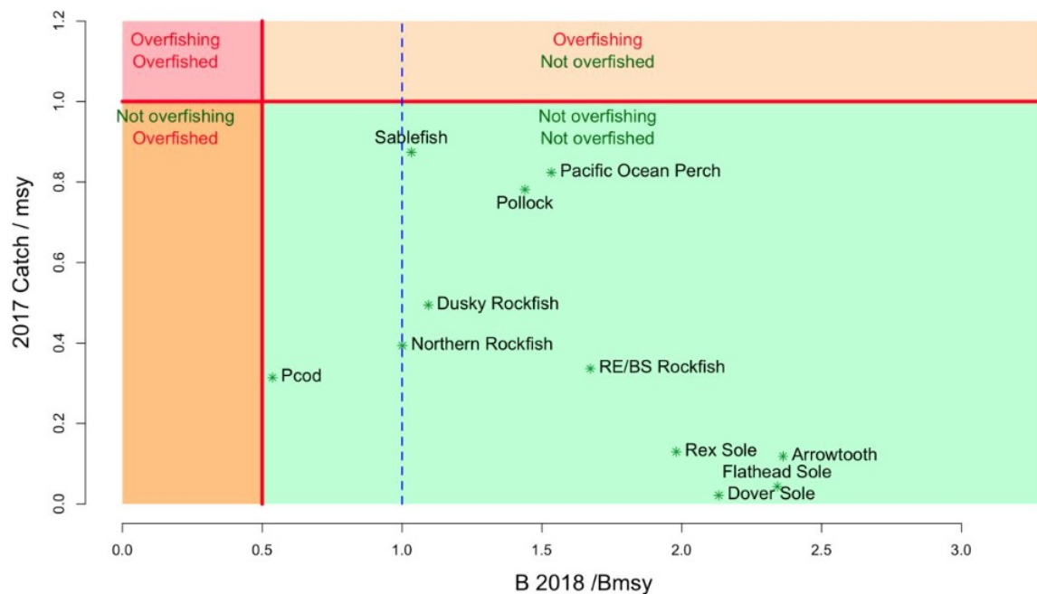
Figure 71 Summary of Gulf of Alaska stock status next year (spawning biomass relative to BMSY; horizontal axis) and current year catch relative to fishing at Fmsy (vertical axis). Note that sablefish is for Alaska-wide values including the BSAI catches (NPFMC 2017a).
