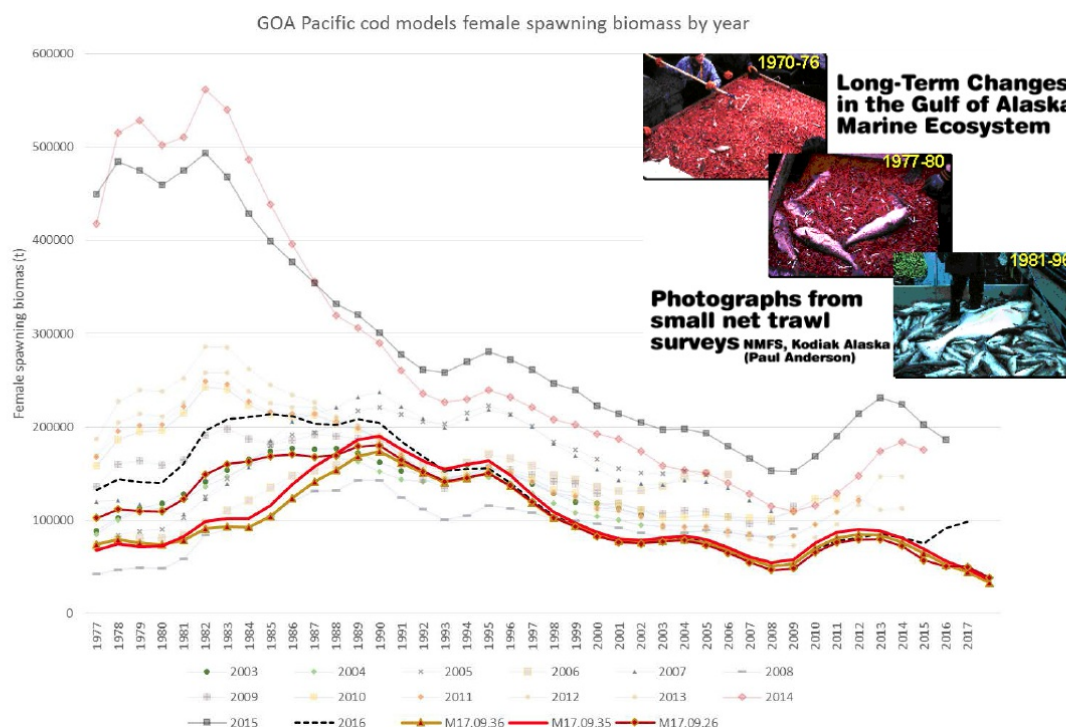
Figure 32 1977-2016 GOA Pacific cod female spawning biomass from the 2003 through the 2016 stock assessments with the authors's preferred models M17.09.35,36, 26, and (inset) images from the NMFS small net survey off Kodiak Alaska showing change in species composition over time (Barbeaux et al. 2017).
