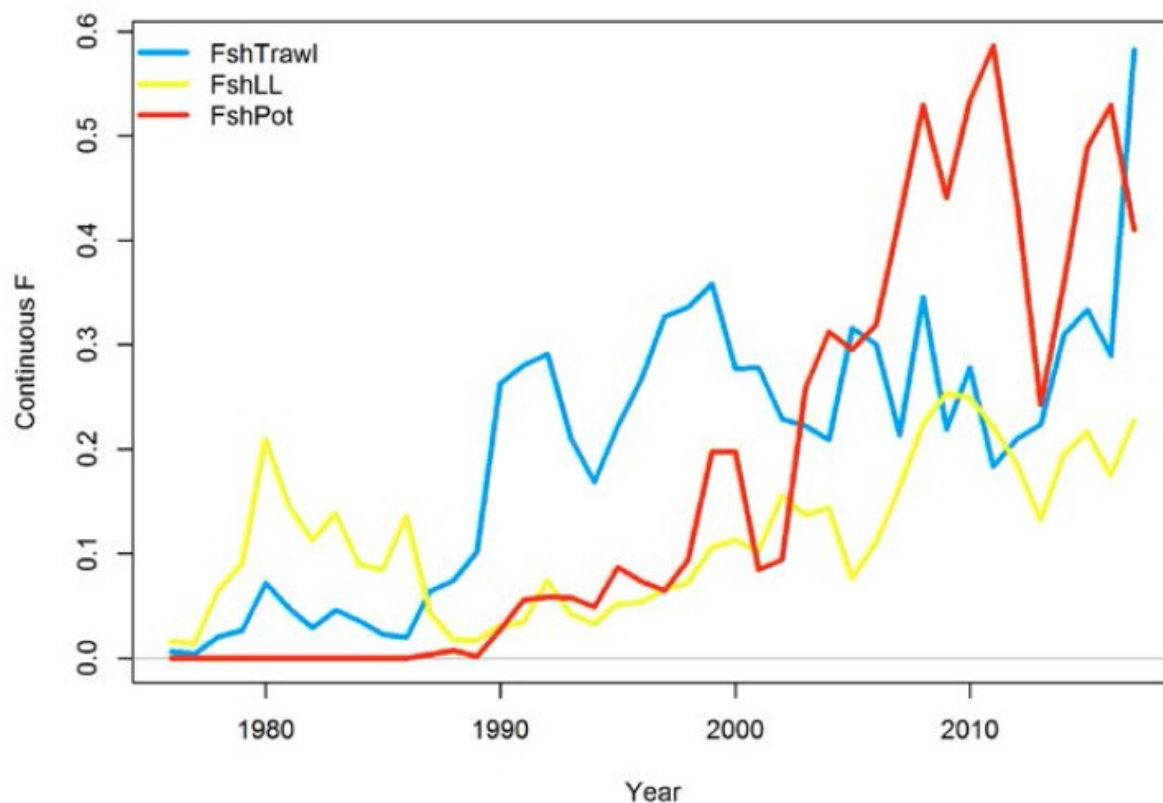
Figure 30 Estimated fishing mortality by trawl, longline, and pot GOA Pacific cod fisheries (Barbeaux et al. 2017).
