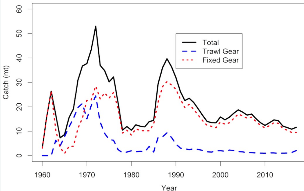
Figure 60 Sablefish catch by gear type (Hanselman et al. 2017).
