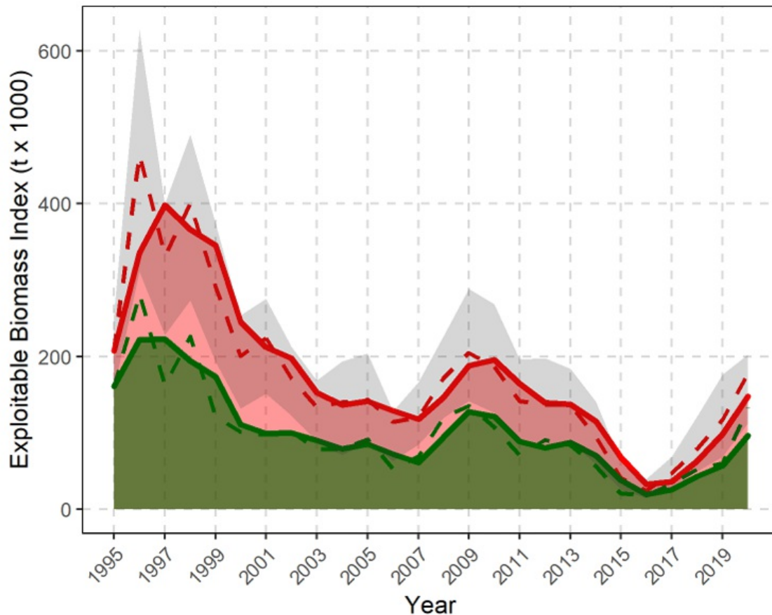
Figure 6: Trawl survey exploitable biomass indices (t × 1000) by shell condition for combined Assessment Divisions. Soft-shell and new-shell crab represent recruitment (green) and intermediate and old-shell crab represent residual biomass (red). Dashed lines shows annual estimates and solid lines are the 2-year moving average estimates. Shaded grey 95% confidence intervals apply to annual estimates. From (DFO 2022b).
