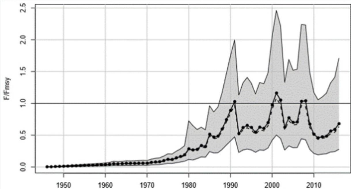
Figure 9 Estimated time series of F relative to F_{MSY} . Solid line indicates estimates from base run of the Beaufort Assessment Model; dashed lines represent median values; gray error bands indicate 5th and 95th percentiles of the MCB trials. Source: (SEDAR 2018a)
