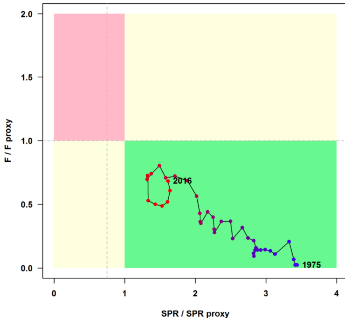
Figure 5 Stock synthesis estimates of spawning output (x-axis) and fishing mortality (y-axis) relative to provisional reference levels of SPR30%, for St. Thomas/St. John. The vertical gray dotted line shows the reference level associated with Minimum Stock Size Threshold (MSST) and the horizontal gray dotted line shows the Maximum fishing mortality threshold (MFMT) (from SEDAR 2019).
