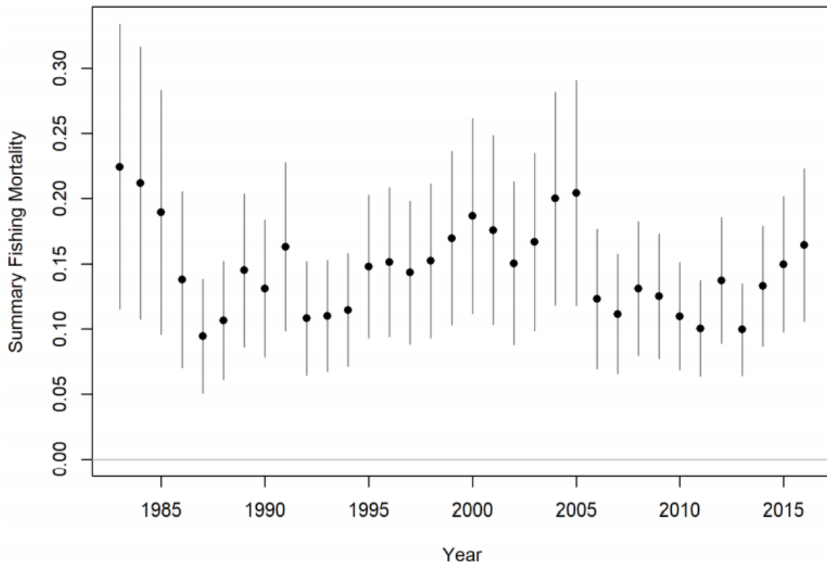
Figure 6 Puerto Rico, proportion of the stock killed by fishing (i.e., harvest rate in biomass landed / total biomass) and associated 95% confidence intervals (vertical lines).
