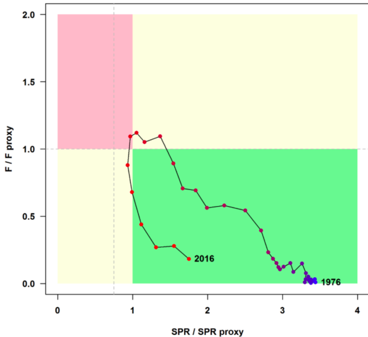
Figure 4 Stock synthesis estimates of spawning output (x-axis) and fishing mortality (y-axis) relative to provisional reference levels of SPR30%, for St. Croix. The vertical gray dotted line shows the reference level associated with Minimum Stock Size Threshold (MSST) and the horizontal gray dotted line shows the Maximum fishing mortality threshold (MFMT) (from SEDAR 2019).
