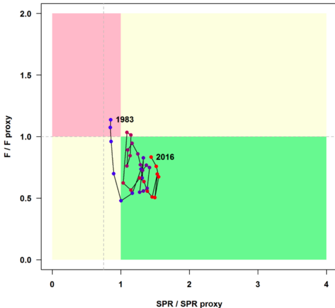
Figure 3 Stock synthesis estimates of spawning output and fishing mortality relative to provisional reference levels of SPR30%, for Caribbean spiny lobster in Puerto Rico (from SEDAR 2019).
