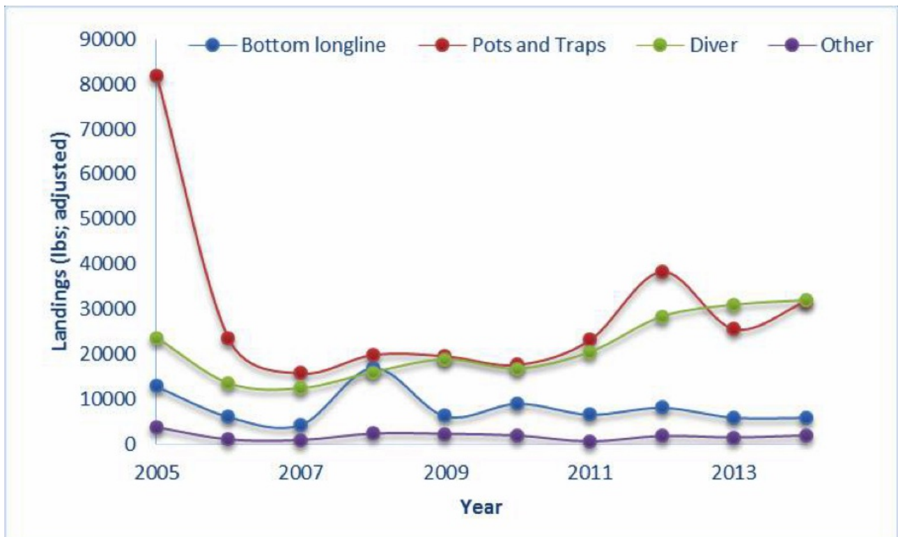
Figure 1 Landings of queen triggerfish by gear type from Puerto Rico (2005–2014). Data provided by David Gloeckner, NOAA. Data are adjusted for known underreporting. Partial landings data are reported here; confidential landings are not included.
