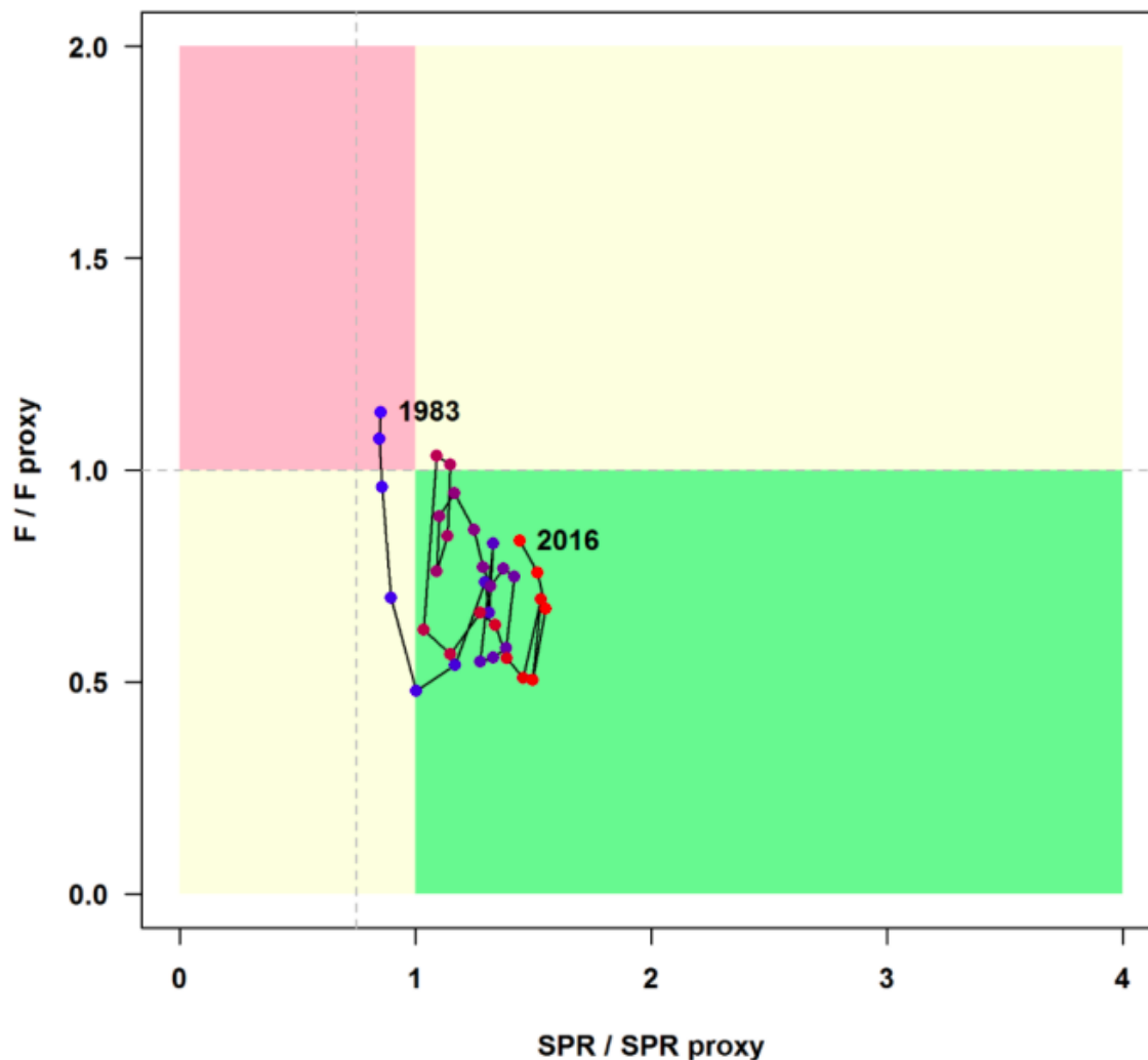
Figure 7 Stock synthesis estimates of spawning output and fishing mortality relative to provisional reference levels of SPR30%, for Caribbean spiny lobster in Puerto Rico (from SEDAR 2019).
