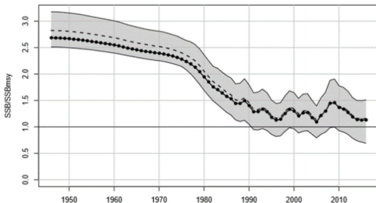
Figure 8 Estimated time series of spawning biomass relative to SSBMSY. Solid line indicates estimates from base run of the Beaufort Assessment Model; dashed lines represent median values; gray error bands indicate 5th and 95th percentiles of the MCB trials. Source: (SEDAR 2018a)
