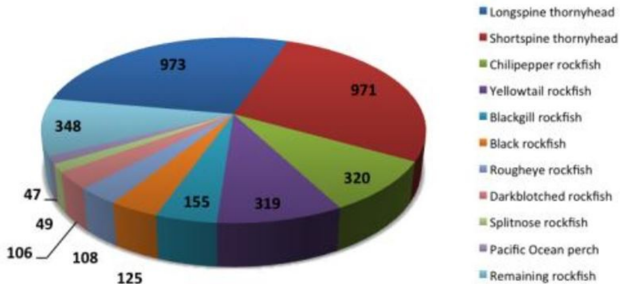
Figure 3: Species composition of thornyhead and rockfish catch in the non-hake commercial groundfish fisheries, 2011 (tons) (Bellman et al. 2012).
