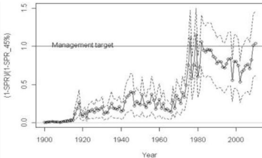
Relative Spawning Potential Ratio ( 1-SPR/1-SPR_{45\%} ), with 95% confidence intervals. A relative SPR value of >1.0 indicates overfishing for that year. (Figure from Stewart, I.J., Thorson, J.T., and Wetzel, C. 2011).
