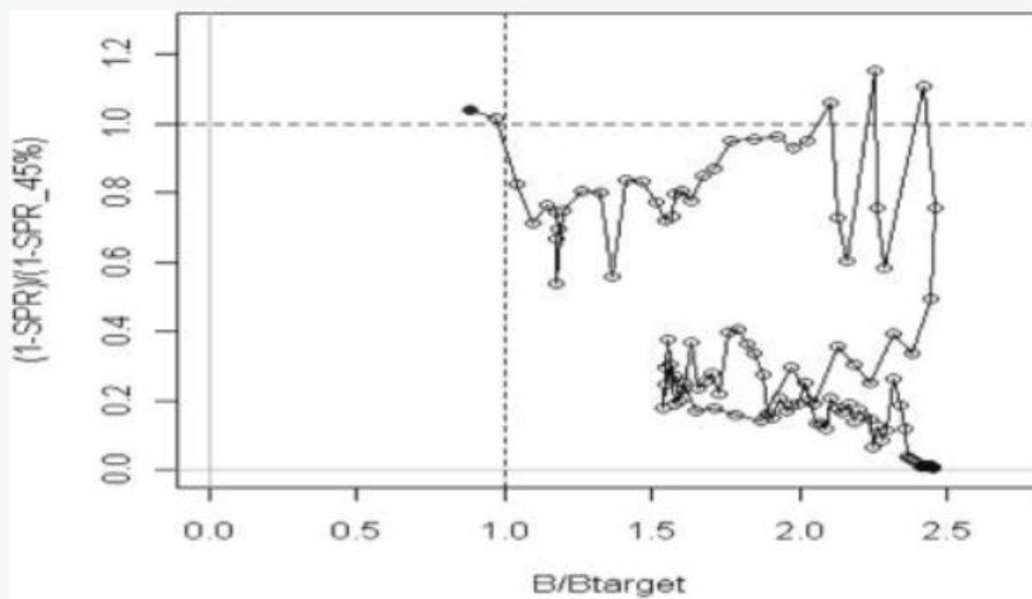
Fishery exploitation, expressed as Relative SPR ( 1-SPR/1-SPR_{45\%} ), compared to stock status ( SB/SB_{40\%} ) (Figure from Stewart, I.J., Thorson, J.T., and Wetzel, C. 2011).
