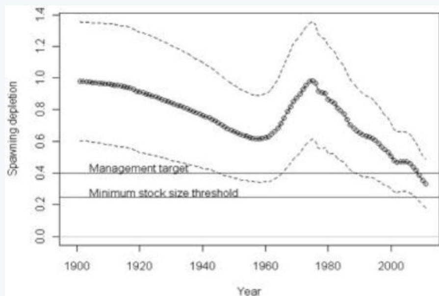
Figure 18: Estimated sablefish spawning biomass relative to SB_0 , with 95% confidence intervals (figure from Stewart, I.J., Thorson, J.T., and Wetzel, C. 2011).
