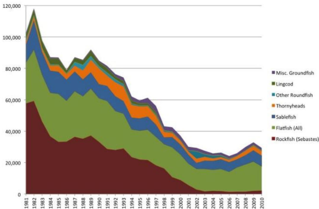
Figure 1: Composition of recent groundfish catches, 1981-2010 (Data from PFMC 2014).
