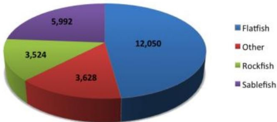
Figure 2: Composition of the catch in the non-hake commercial groundfish fisheries, 2011 (tons) (Bellman et al. 2012)
