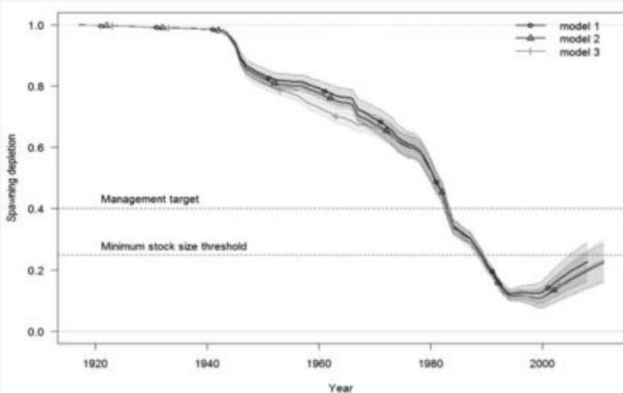
Modeled estimates of canary rockfish spawning biomass relative to SB_0 (Figure from Wallace and Cope 2011).
