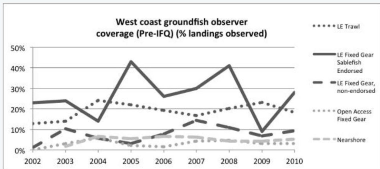
Figure 23: Observer coverage of west coast groundfish landings, 2002-2010 (Data source: WCGOP 2012).
