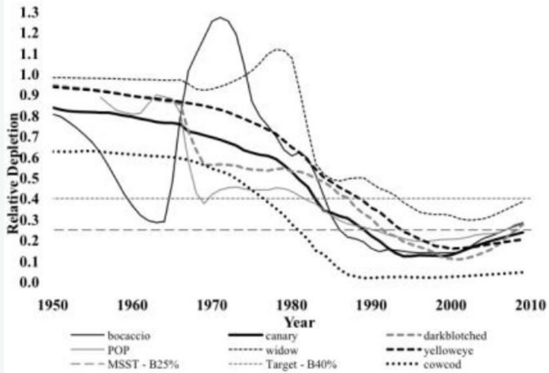
Estimated spawning biomass relative to SB0 for seven 'overfished' rockfish species (Figure fromPFMC 2011a).
